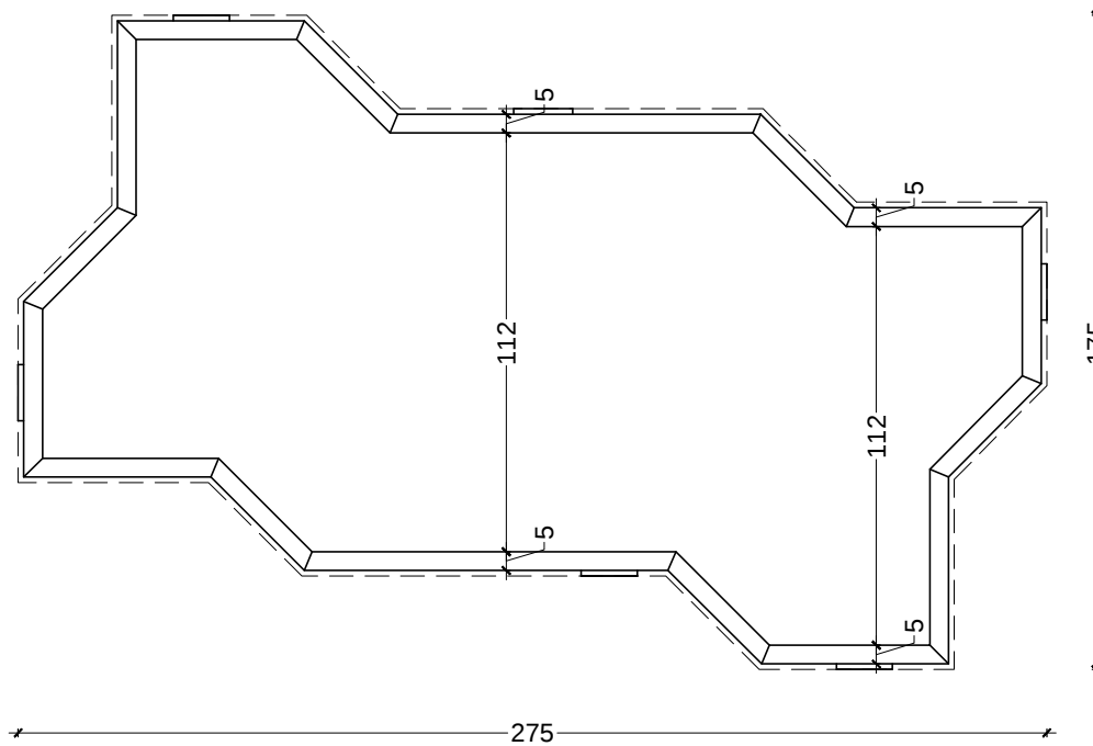
Plan (Scale :- 1 : 2)
